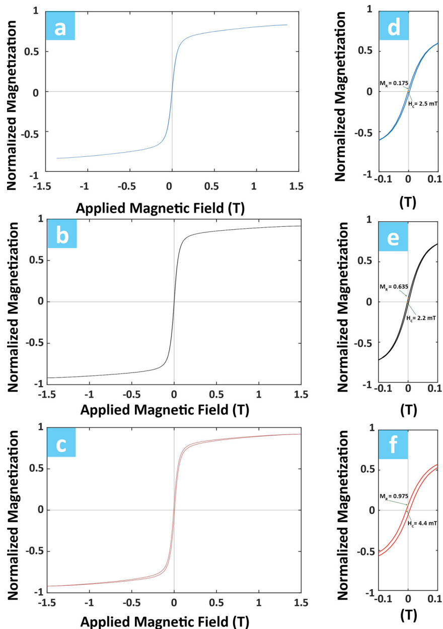
Fig. 3 Magnetic hysteresis. Magnetic hysteresis results for a seafloor white pumice b Havre white raft pumice and c pink raft pumice with d-f close ups of the origin of the magnetic hysteresis results highlighting subtle differences in magnetic remanence ( M_R ) and coercivity ( H_C ) between the different pumice types. A combination of magnetic parameters (Supplementary Table S3) and frequency dependence of magnetic susceptibility ( \chi_{fd} ) are utilized to determine that the white and pink raft pumice hysteresis loops represent a mixture of superparamagnetic (SP) < 10 nm and MD magnetite grains, and that seafloor white pumice contains purely MD magnetite. In addition, c, f Havre pink raft pumice displays a classic wasp-waisted hysteresis signature closing past 0.6T suggesting that both magnetite and hematite are present 51 . Duplicates for white and pink raft pumice sample type show similar results as displayed here, while limited material of white seafloor pumice allowed for only one analysis.
