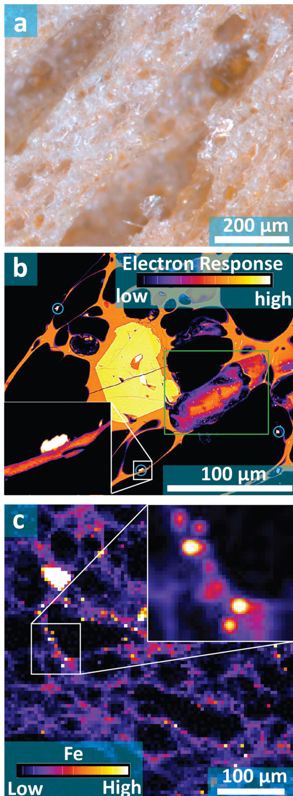
Fig. 2 Microlites and nanolites on vesicle walls in natural pink pumice.
